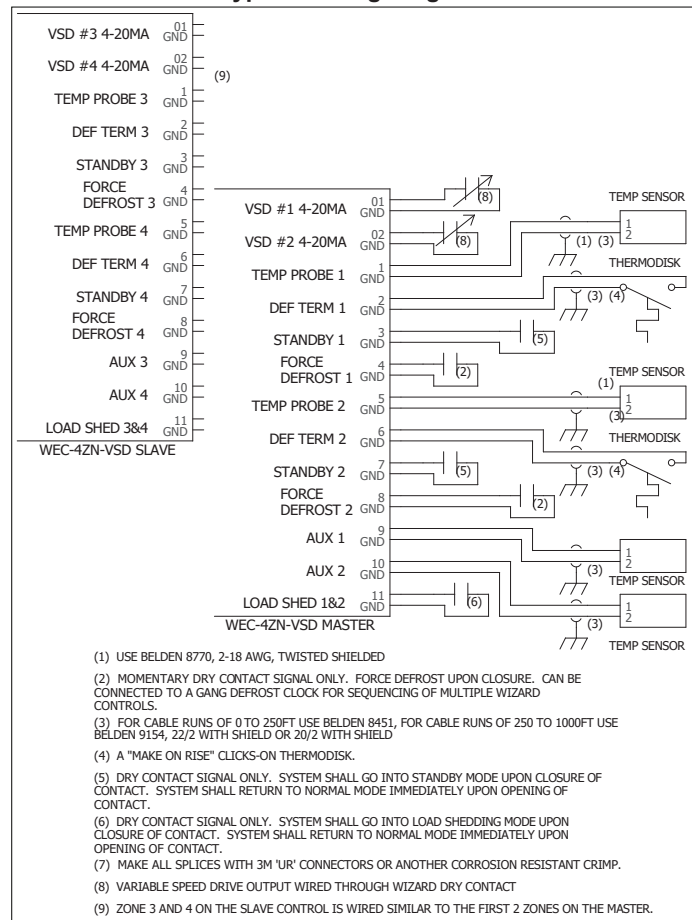
Typical Wiring Diagram
